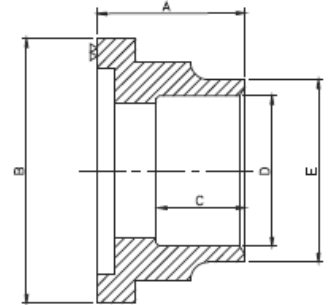
Suction and discharge bushings
